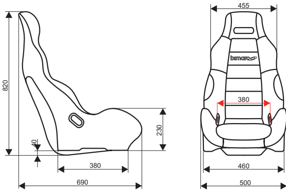
Model: BRAVO Construction: Polyester-Fiberglass Weight: 6,5 kg
